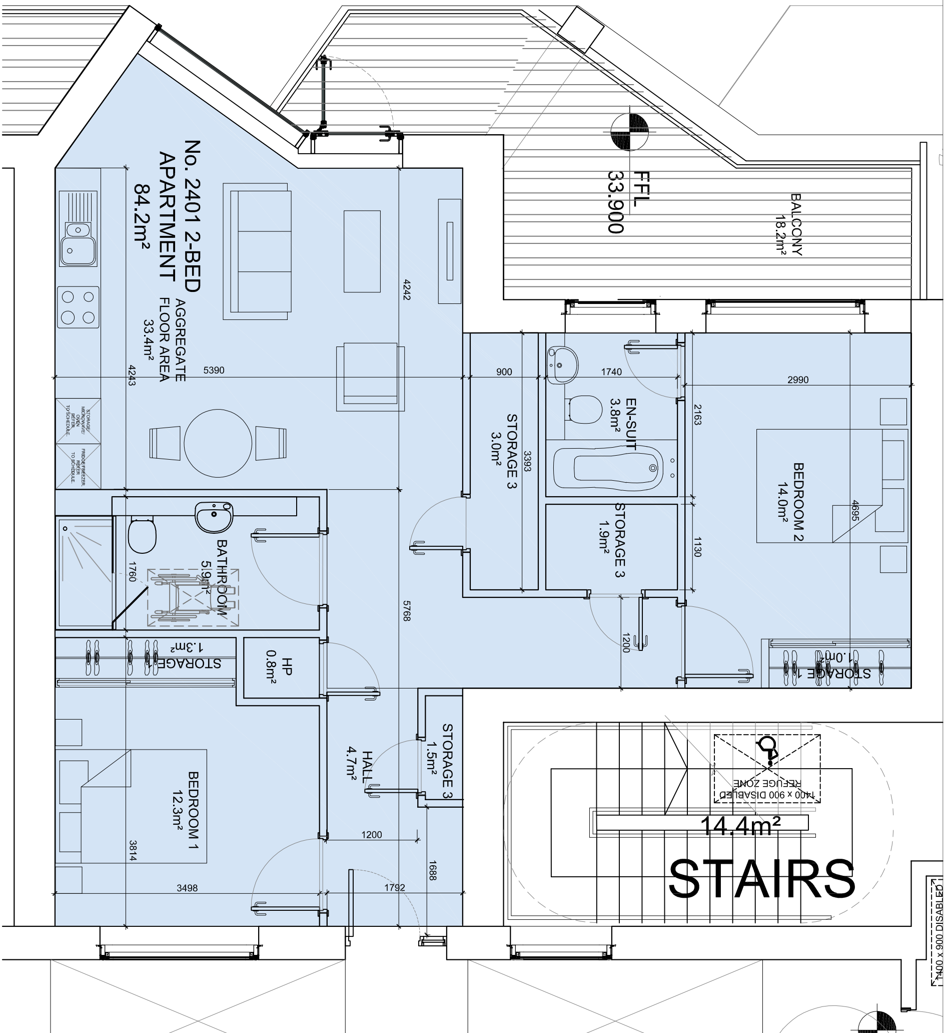
TYPICAL 2-BED APARTMENT PROPOSED SCHEME (TYPE R)
